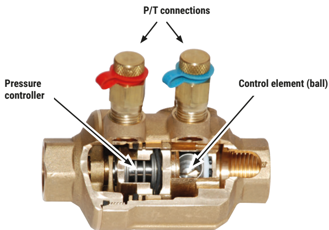
Fig. 9: Components of a mechanical PI valve, e.g. a PIQCV.
