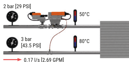
Fig. 107: FCU, with BMS-corrected heating setpoint and required flow rate.
