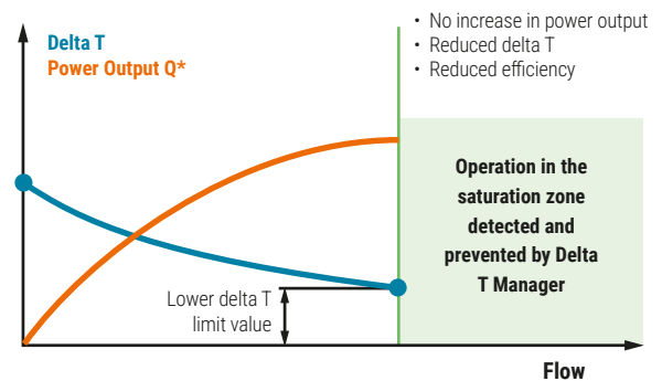
Fig. 59: Improved energy efficiency with the Energy Valve™ delta T manager enabled.
