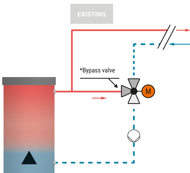
Fig. 123: Boiler with globe valve.
