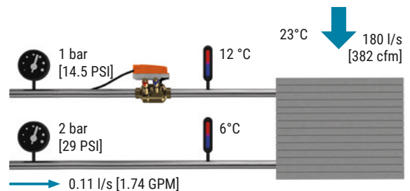
Fig. 85: FCU at design operation.
