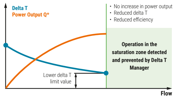
Fig. 114: Delta T manager
