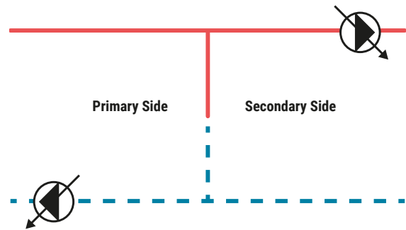
Fig. 53: Simple representation of a primary/secondary circuit with a hydronic deflector.
