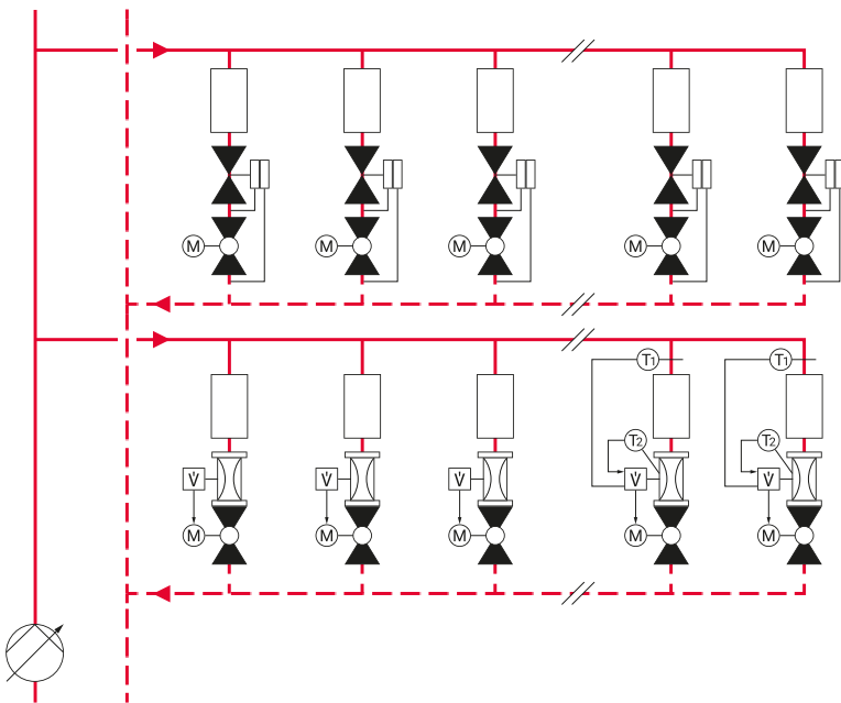
Fig. 20: Energy efficiency class A (DIN EN ISO 52120-1) Optimum operation thanks to pressure-independent flow control of individual consumers (Energy Valve in flow control or power control operating mode).
