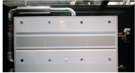
Fig. 90: Ceiling-integrated chilled beam with air and chilled water supply.
