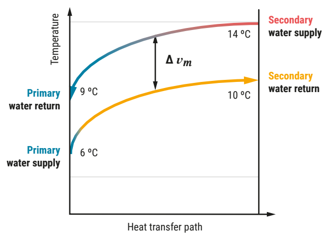
Fig. 76: \Delta\vartheta_m mean differential temperature with saturation.
