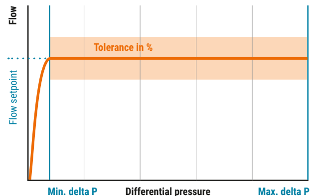
Fig. 57: Dynamic balancing ensures an accurate flow rate.
