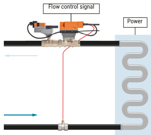
Fig. 28: Power control of the energy input to a consumer.
