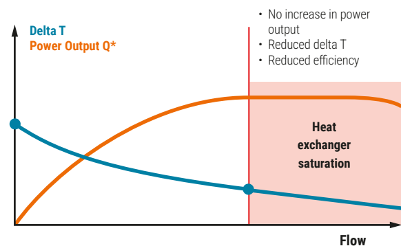
Fig. 58: Low delta T syndrome
