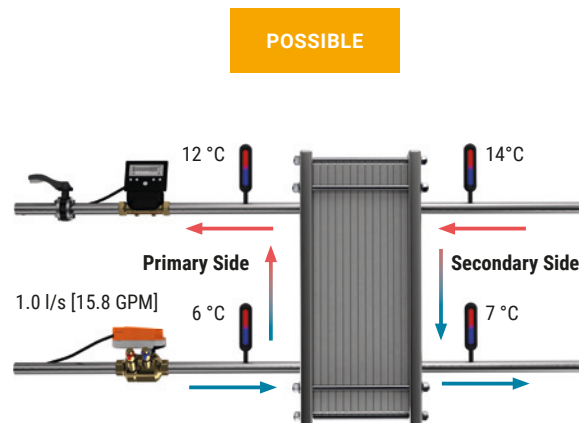
Fig. 77: Dynamic balancing.
