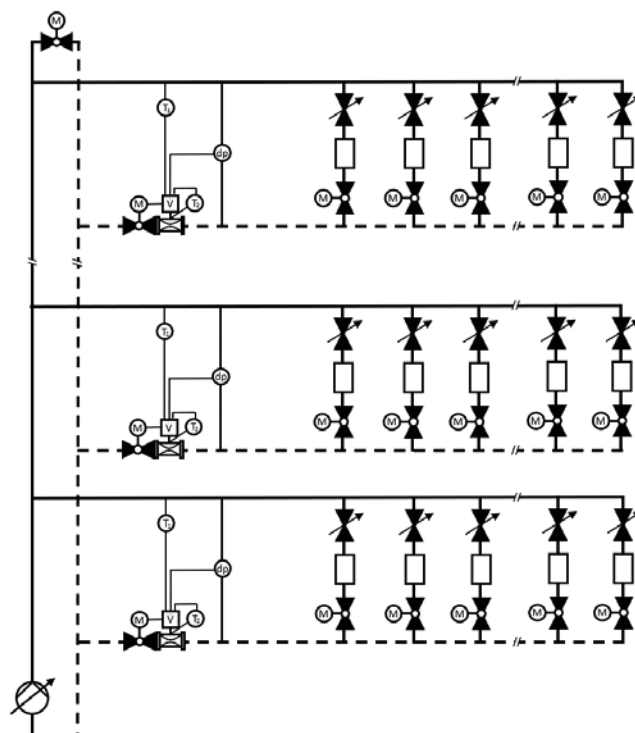
Fig. 37: Dynamic balancing of the system segment (building floor) and static balancing of the consumers.
