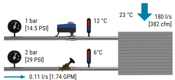
Fig. 83: FCU at design operation.
