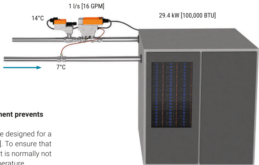
Fig. 118: CRAC device under "design load conditions".
