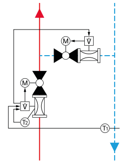
2-way Energy Valve with 2-way EPIV, DN 15...150
