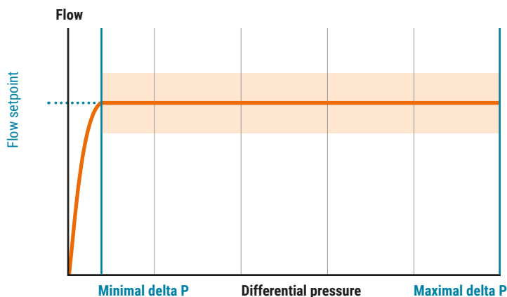
Fig. 11: Improved sturdiness with mechanical PI valves.
