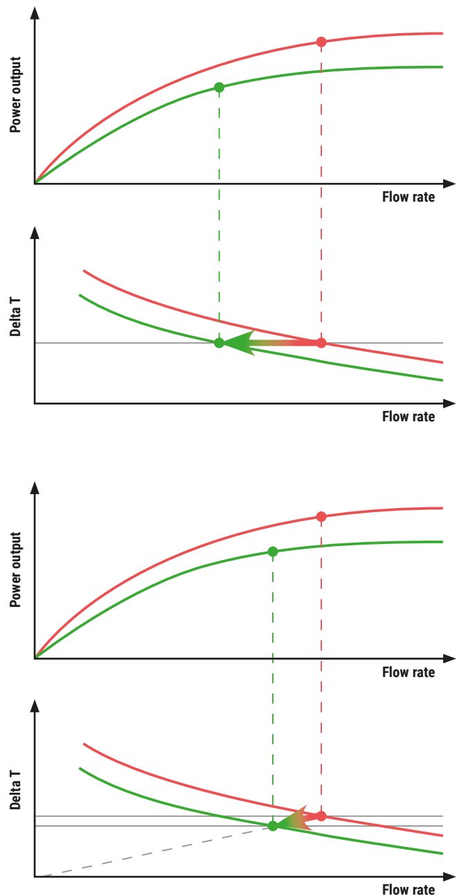
Fig. 35: Delta T manager scaling.
