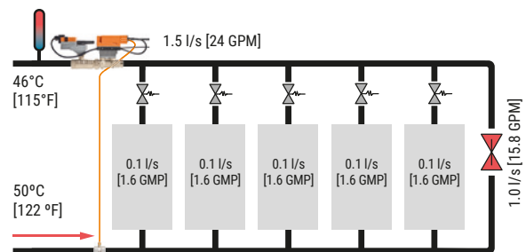
Fig. 112: With an Energy Valve, not only leaking short-stroke globe valves but also an open bypass can be clearly identified.
