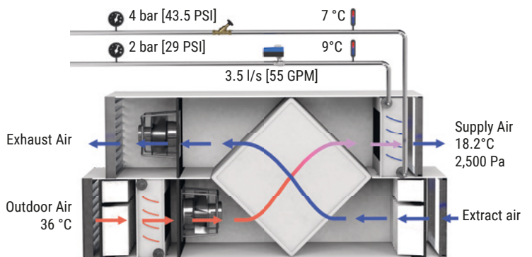
Fig. 61: AHU with valve overflowing.
