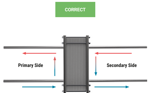
Fig. 71: Cooling transfer station connected in contraflow.
