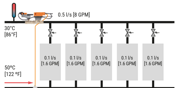
Fig. 110: With a Belimo Energy Valve™, the flow in the branch can be measured when each valve is opened, allowing verification.
