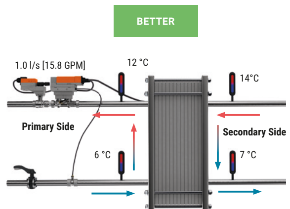
Fig. 78: Dynamic balancing with power characteristic monitoring.
