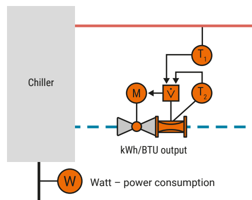
Fig. 127: Chiller with cooling circuit.
