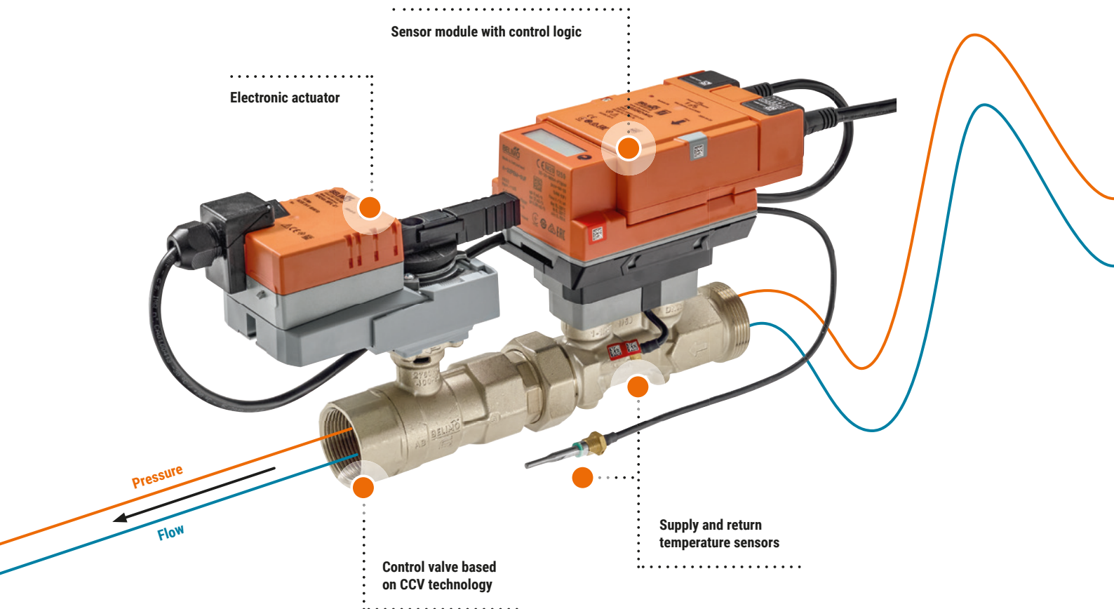
Fig. 12: Belimo electronic PI valve, e.g. a Belimo Energy Valve™.
