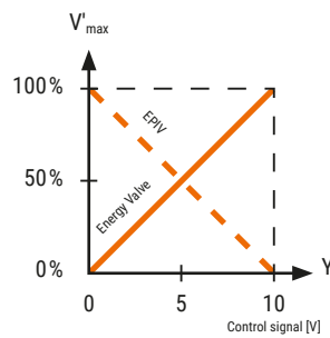
Characteristic curve of the Energy Valve (path A) and inverted characteristic curve of the EPIV (path B)
