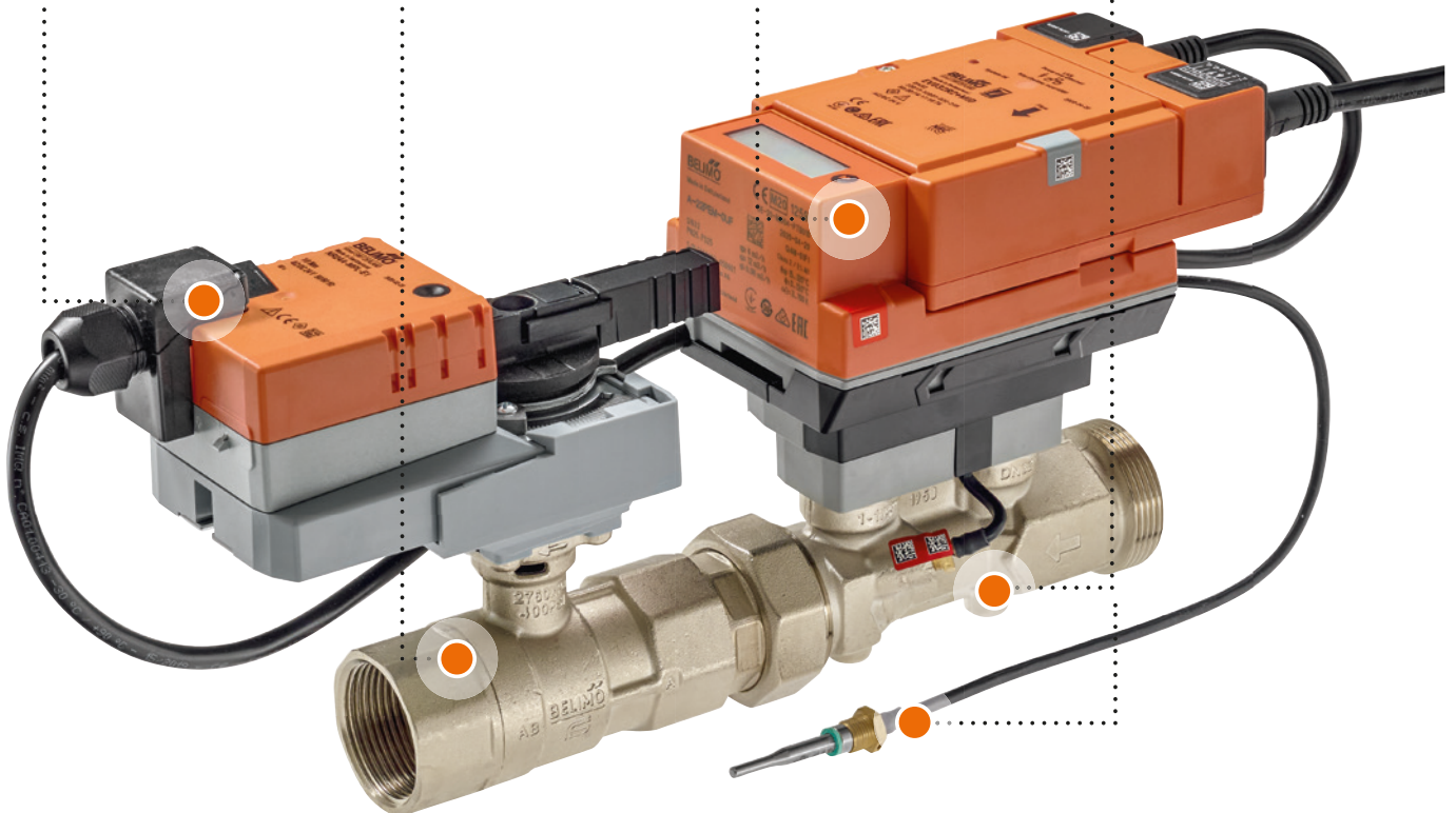
Fig. 24: The components of the Belimo Energy Valve™.
