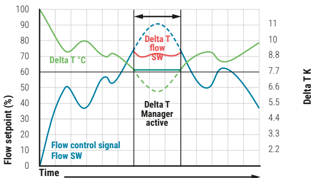
Fig. 33: The delta T manager detects a low delta T, becomes active, and reduces the flow to ensure the minimum delta T.
