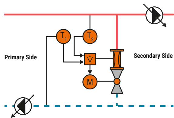
Fig. 54: An Energy Valve that monitors the temperature spread of the primary part and the flow via the hydronic deflector.
