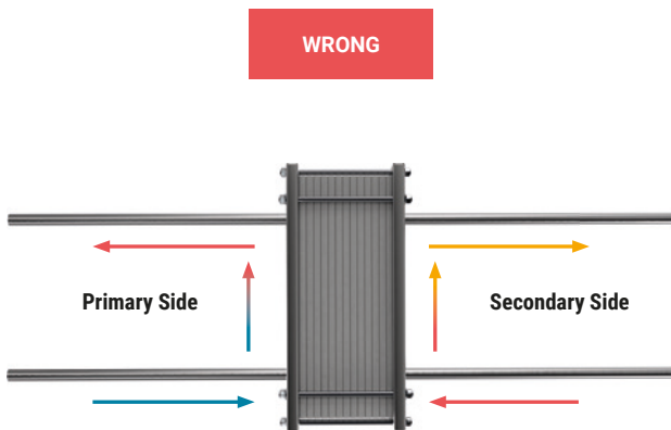
Fig. 69: Cooling transfer station connected in direct current.
