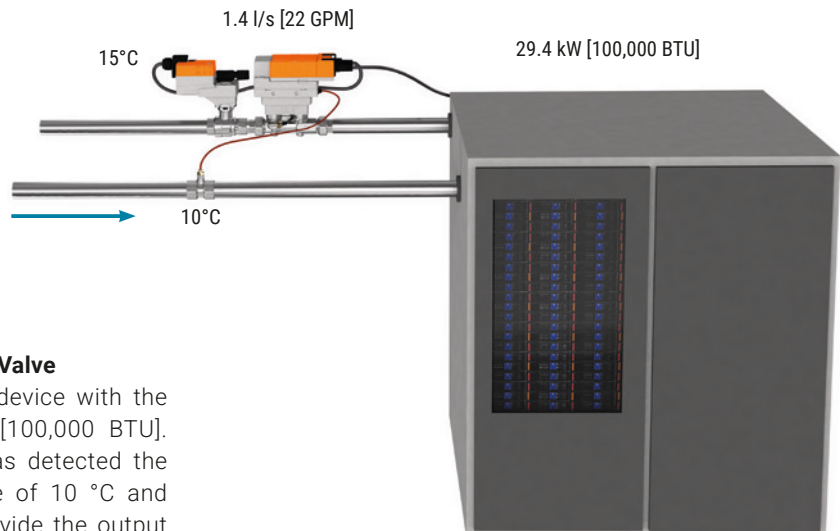
Fig. 119: CRAC device with higher supply temperature to save energy.
