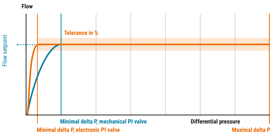
Fig. 13: Electronic PI valves can typically maintain the flow rate at lower delta P than can mechanical PI valves.
