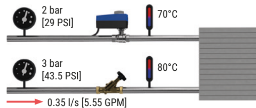
Fig. 104: FCU in heating mode.
