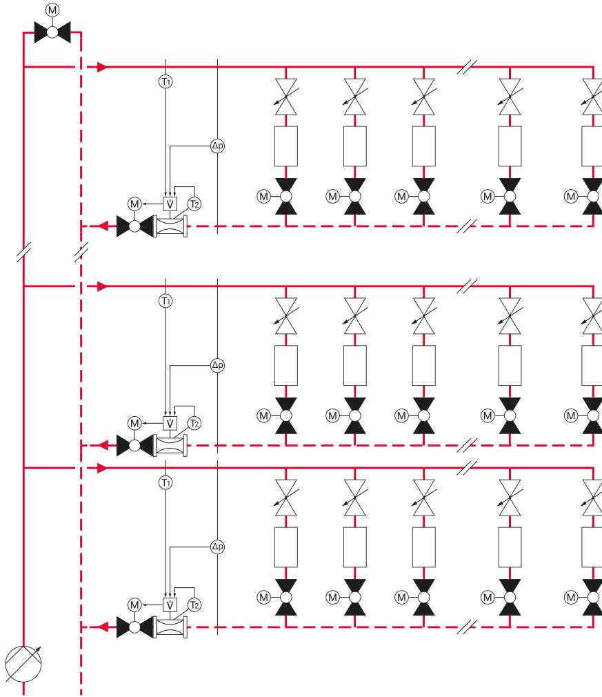
Fig. 22: Energy efficiency class C (DIN EN ISO 52120-1)
