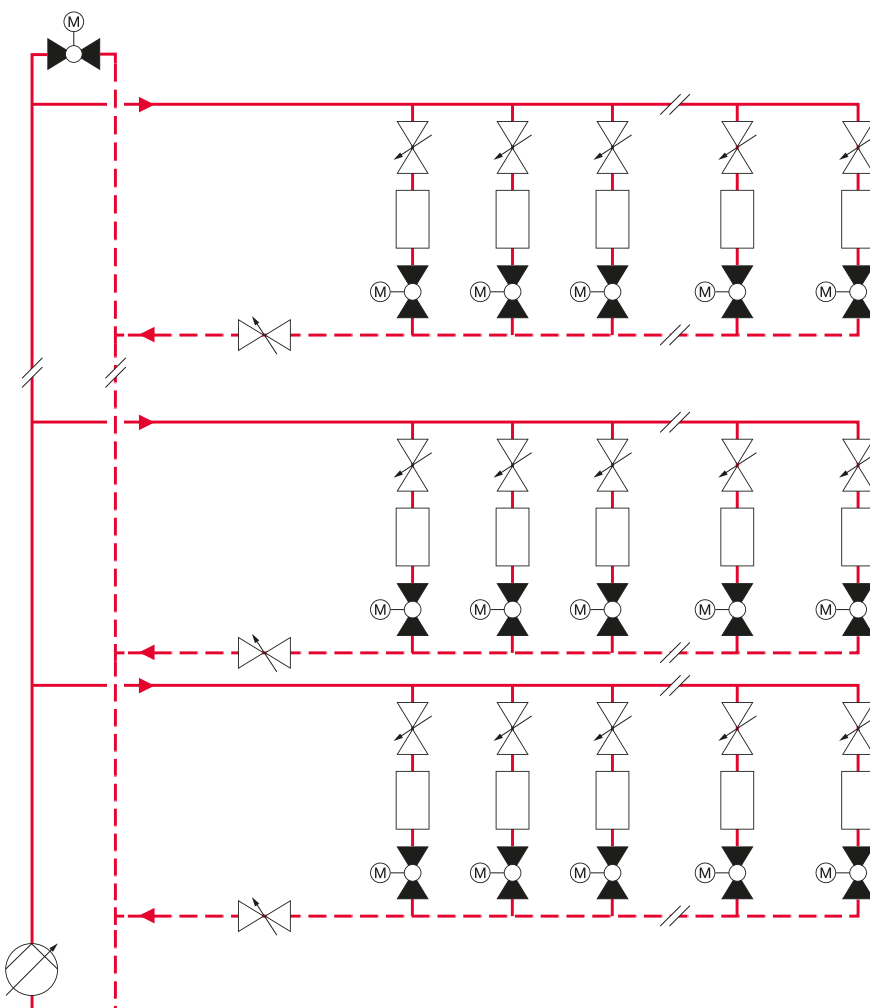
Fig. 21: Energy efficiency class D (DIN EN ISO 52120-1) Lowest energy class with pressure-dependent control valves and static balancing.
