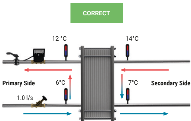
Fig. 73: Typical design flow (cooling application).
