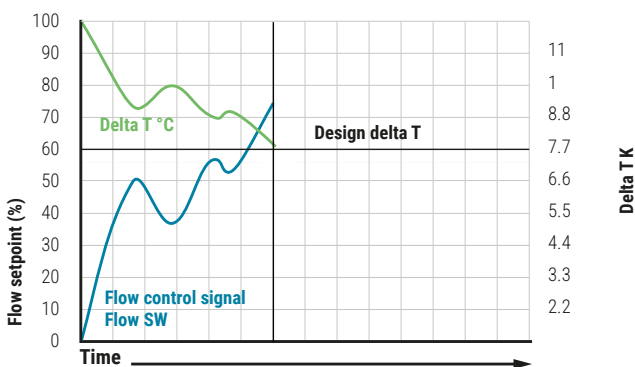
Fig. 31: When the demand increases and the flow changes, the actual delta T starts to decrease.
