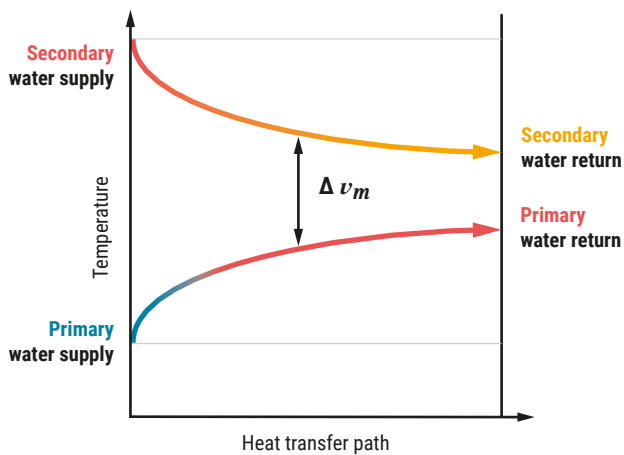
Fig. 70: \Delta\vartheta_m average differential temperature for direct flow.
