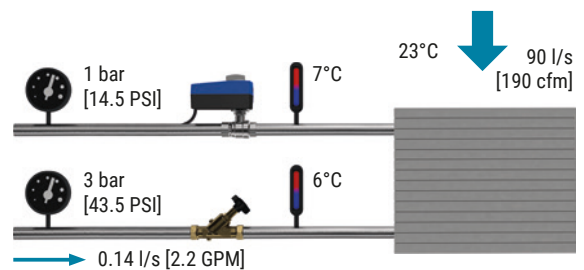
Fig. 84: FCU with valve overflowing.
