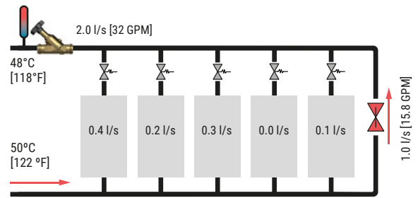
Fig. 111: An accidentally opened bypass valve may be discovered only after weeks, months or even years.
