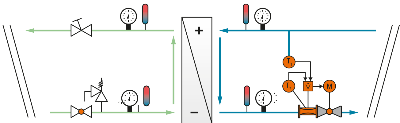
Fig. 68: Supply side (green) and consumer side (blue).
