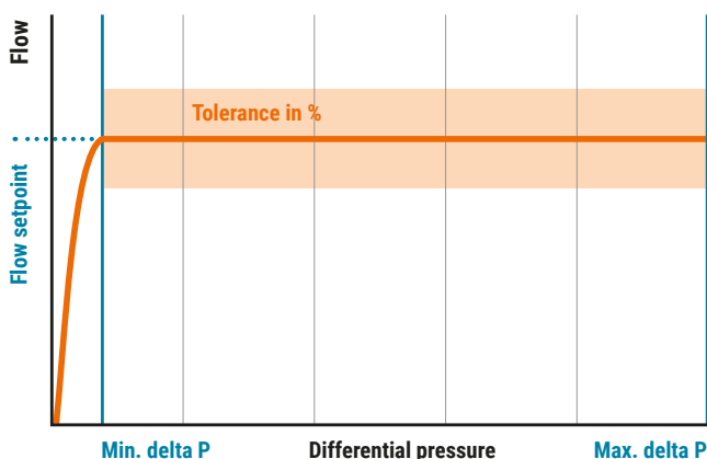
Fig. 92: Dynamic balancing of a chilled beam.
