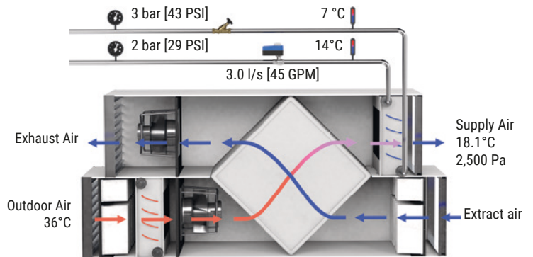
Fig. 60: AHU at design operation.
