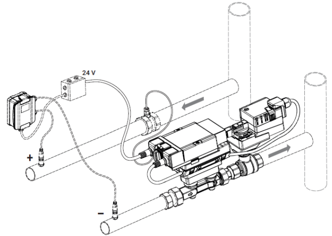
Fig. 39: Installation of 22PDP-18..
