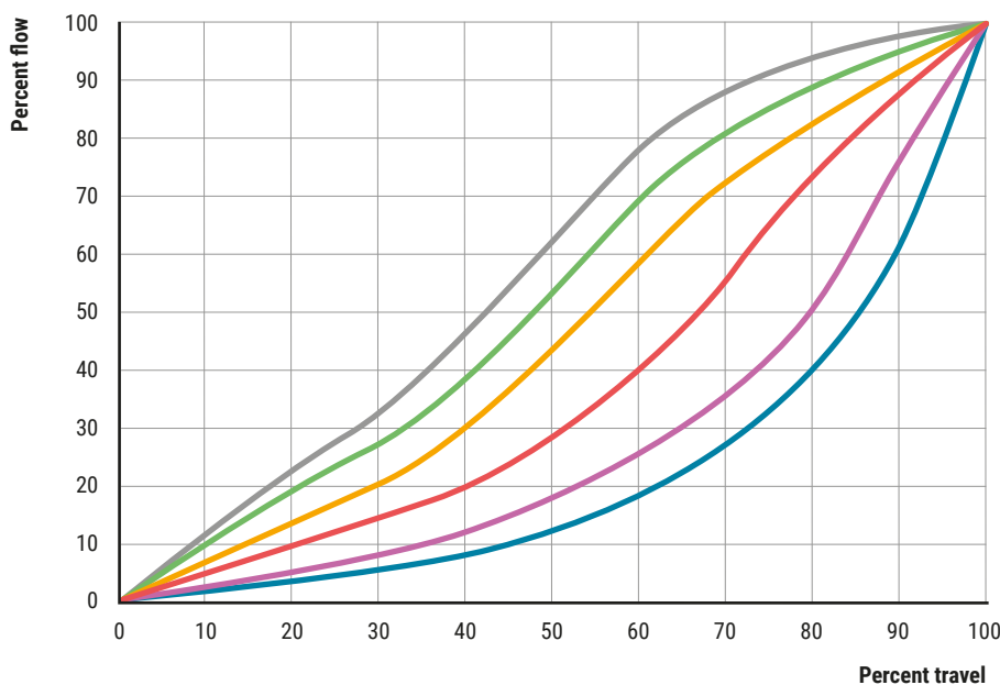
Fig. 25: The distortion of the characteristic curve that could occur if the valve is left in position control.
