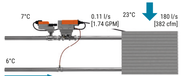
Fig. 86: FCU without too much water.
