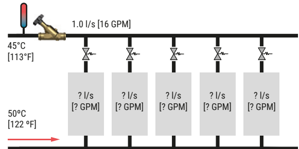
Fig. 109: Mechanical balancing valves allow only static balancing of the total flow, whereby the flow rates to each individual unit are unknown.
