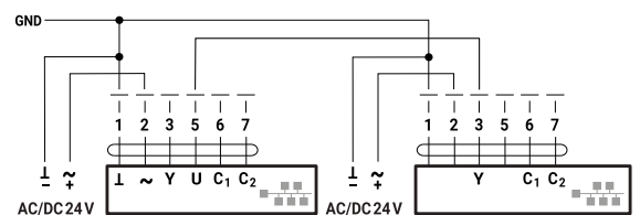
Electrical connection diagram (without analog/bus control)
