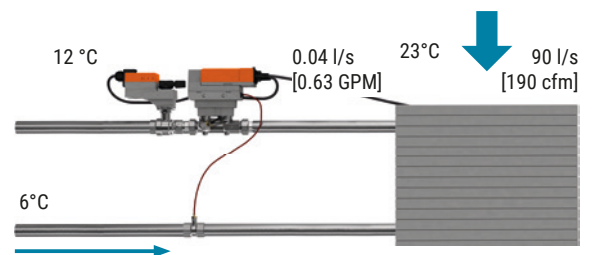
Fig. 87: FCU with delta-T-optimised valve flow.
