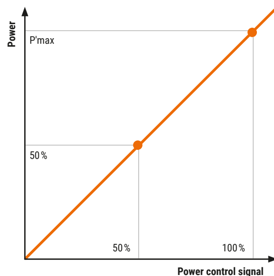
Fig. 29: Control characteristics in power control mode.
