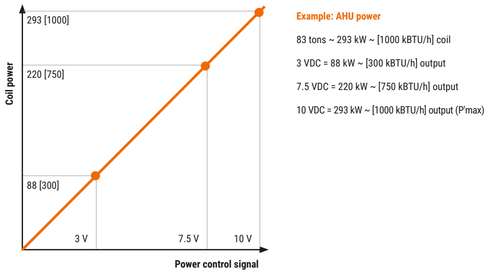
Fig. 30: Example of a coil using power control mode.
