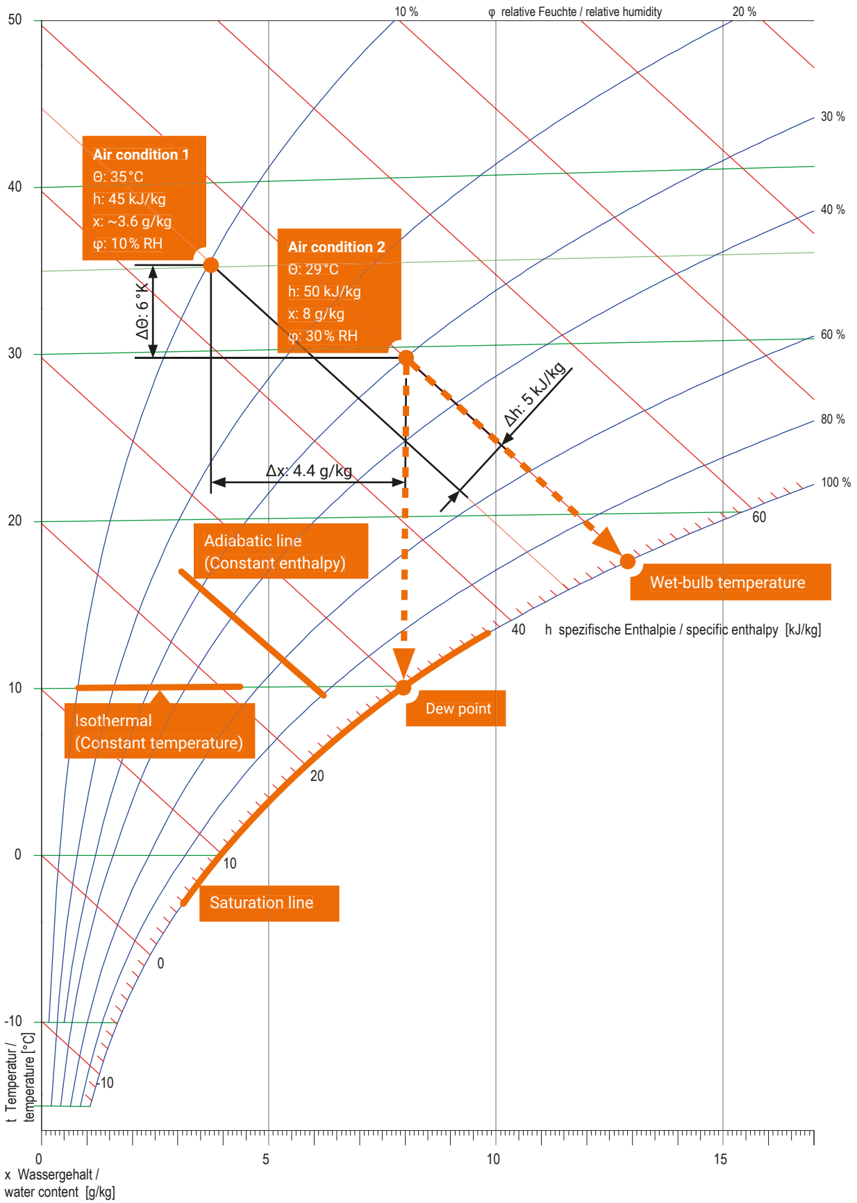
Fig. 95: The dew point depends on the air temperature and the air humidity.
