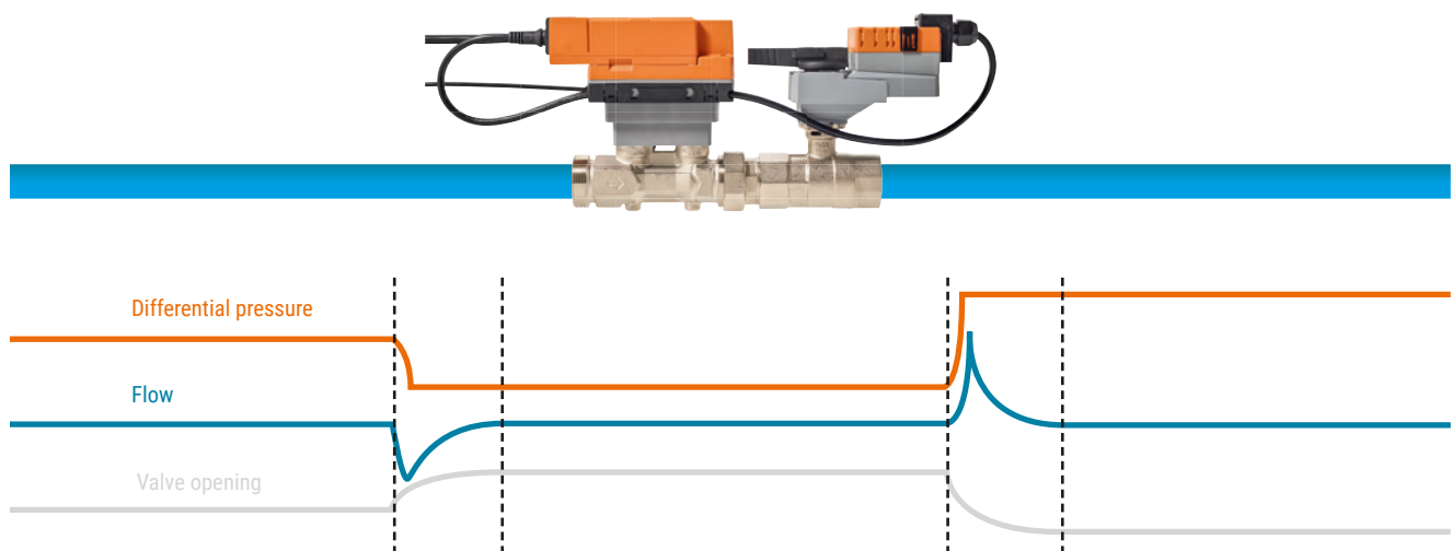
Fig. 15: Compensation of pressure fluctuations by changing the valve opening.
