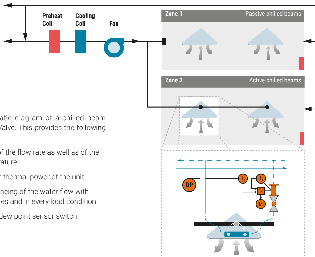
Fig. 91: Chilled beams in a multi-zone system.
