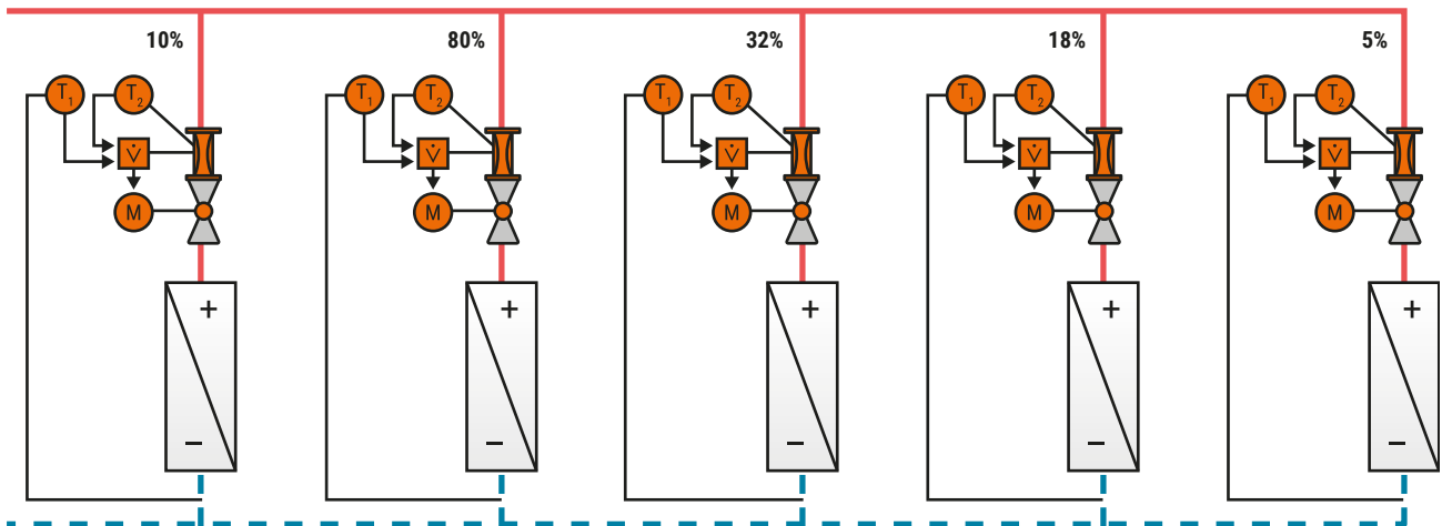
Fig. 52: The largest thermal load is at the valve with the widest opening.
