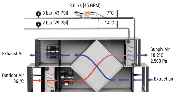
Fig. 62: AHU at design operation.
