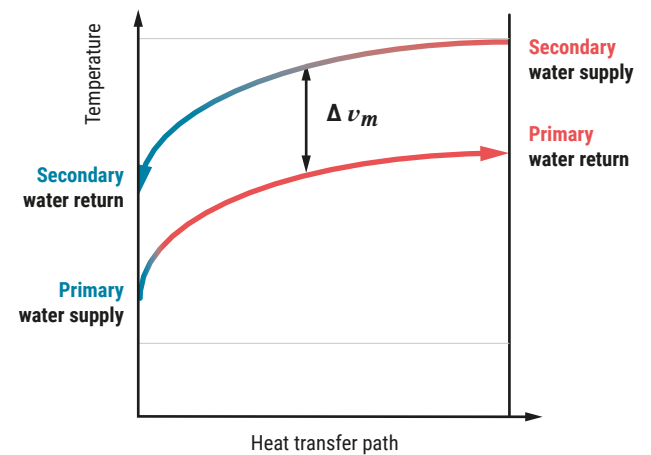
Fig. 72: \Delta\vartheta_m average differential temperature with contraflow.
