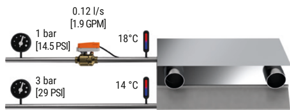
Fig. 97: Chilled beam with a mechanical PI valve.
