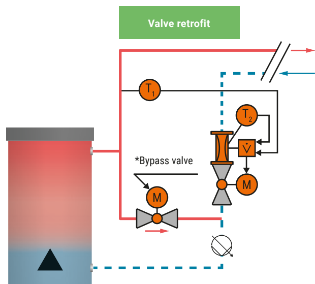
Fig. 124: A non-condensing boiler retrofitted with an air-bubble tight bypass valve and an Energy Valve.
