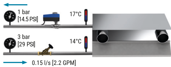
Fig. 96: Chilled beam with a pressure-dependent valve.
