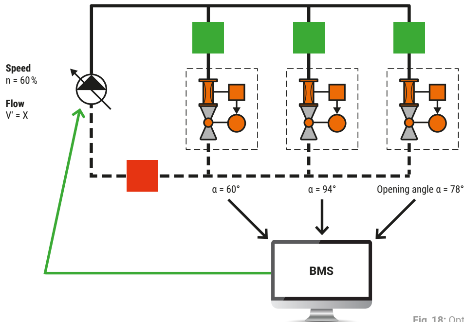
Fig. 18: Optimised operation
