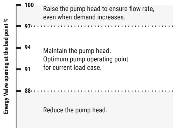
Fig. 17: An example of pump control using the Energy Valve at the bad point.
