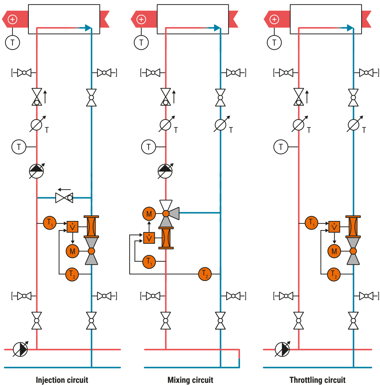
Fig. 125: An overview of the various basic hydronic circuits for heating applications.
