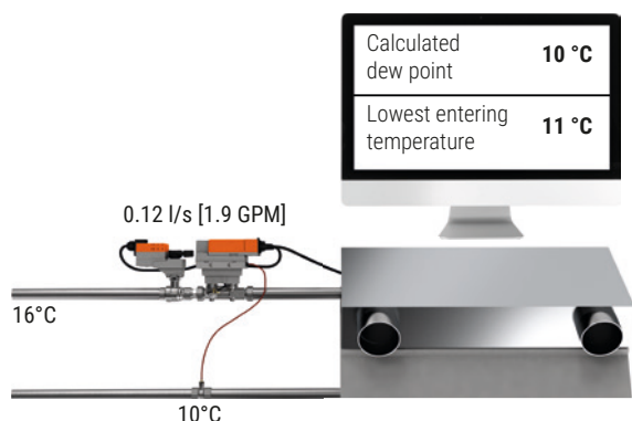
Fig. 99: Chilled beam with an Energy Valve, for which the BMS calculates the dew point using data from a room sensor.
