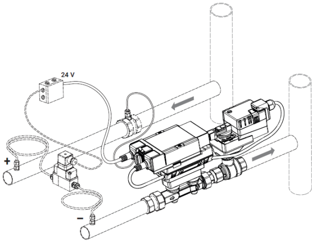
Fig. 38: Installation of 22WDP-11..
