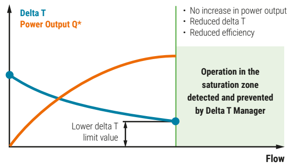
Fig. 102: The Energy Valve's delta T manager guarantees that a minimum delta T is not fallen short of.
