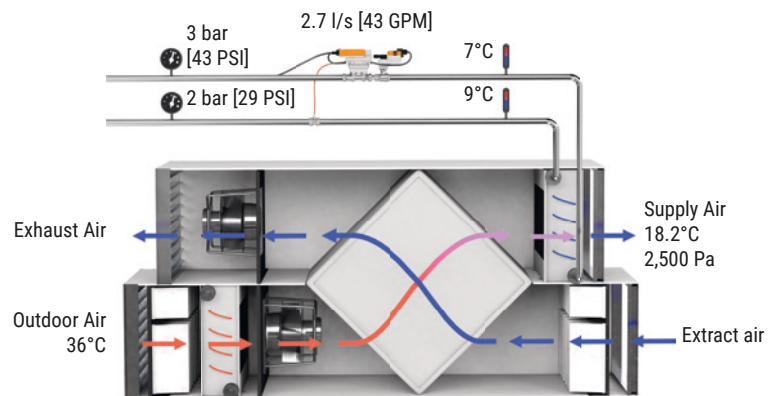
Fig. 63: AHU without valve overflow.
