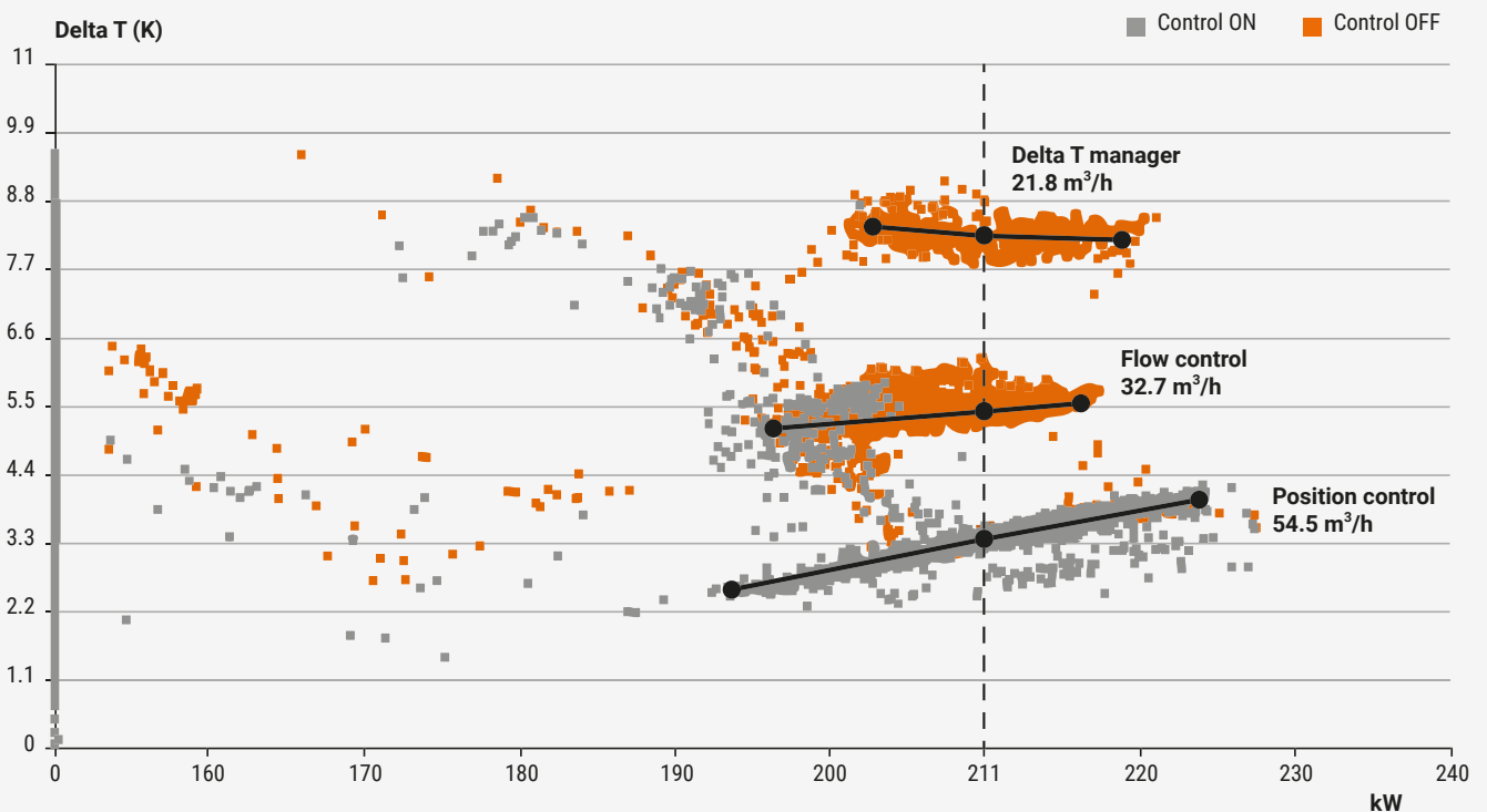
Fig. 34: Operating conditions (delta T and load) of the valve in different control modes.
