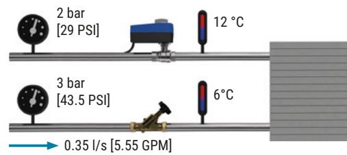
Fig. 103: FCU in cooling mode.
