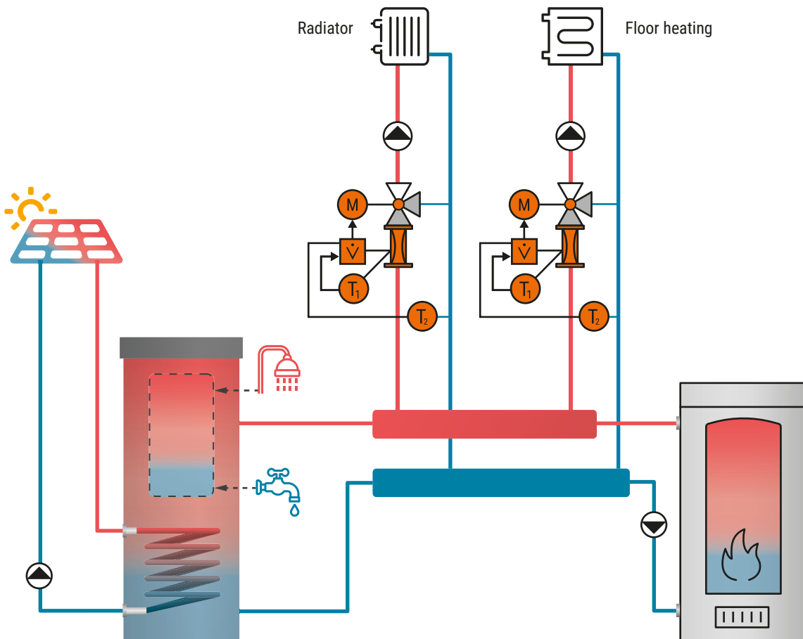
Fig. 122: Typical hydronic diagram of a central heating system combining several alternative and renewable energy sources.
