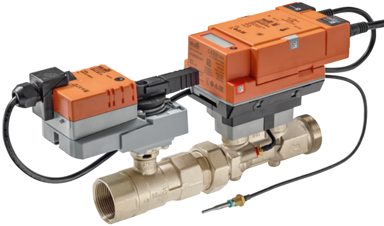
Fig. 55: The Belimo Energy Valve™ 4.
