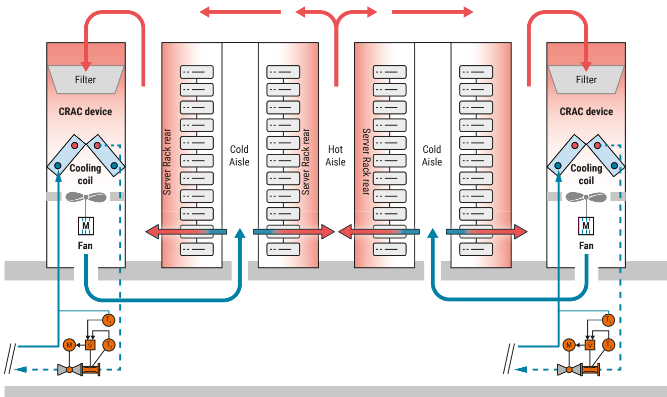
Fig. 117: Schematic of a CRAC device, including airflow to/from the racks.
