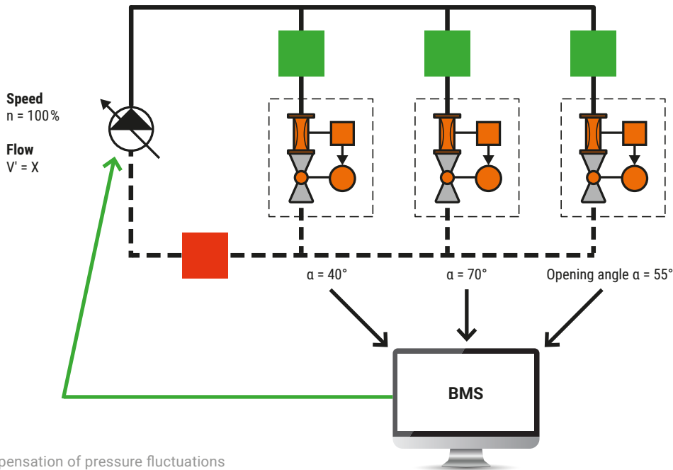
Fig. 16: Compensation of pressure fluctuations by changing the valve opening.
