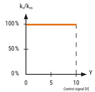
Result: Straight mixing characteristic (path AB)
