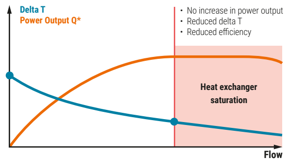
Fig. 113: Low delta T syndrome
