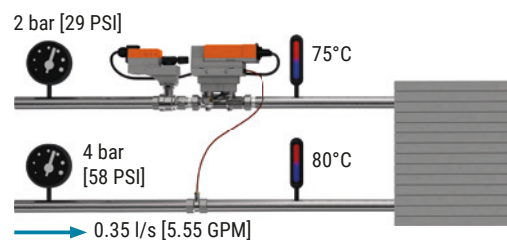
Fig. 106: FCU in heating mode, using a pressure-independent EV.
