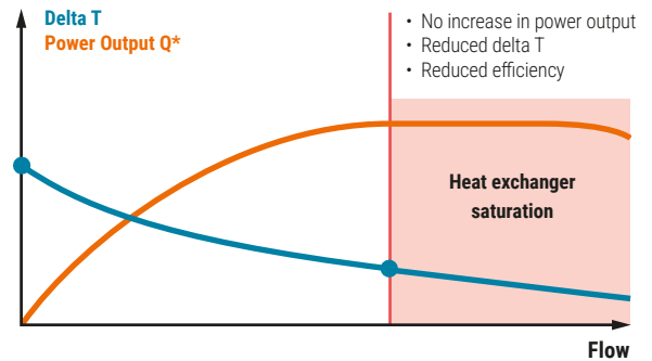
Fig. 101: Low delta T at a consumer (e.g. fan coil).
