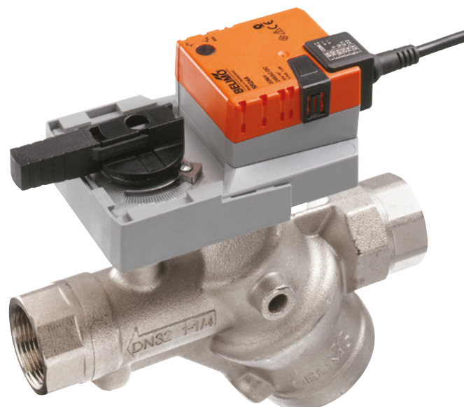
Fig. 8: PICCV, the first Belimo pressure-independent valve.
