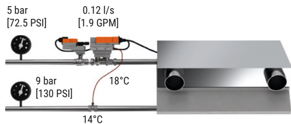
Fig. 98: Chilled beam with an Energy Valve.
