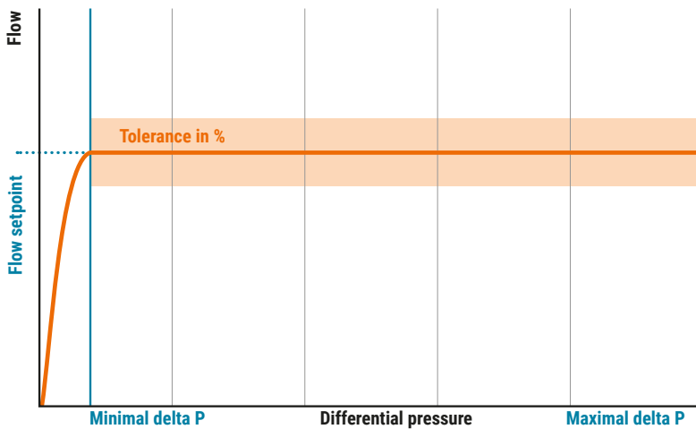
Fig. 82: Dynamic balancing of a FCU.
