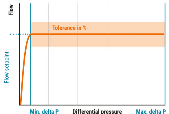
Fig. 27: Control characteristics in flow control mode.
