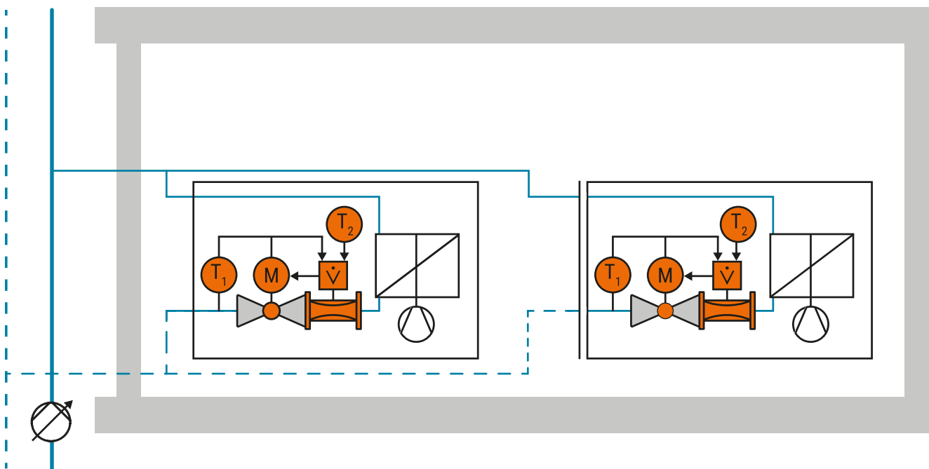
Fig. 81: Typical fan coil application in a single room, with one Belimo Energy Valve™ per fan coil.
