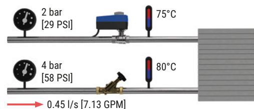
Fig. 105: FCU heating mode and differential pressure increase.
