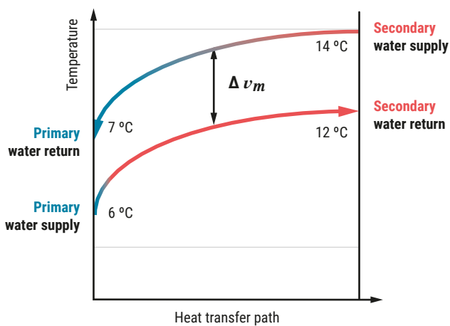
Fig. 74: \Delta\vartheta_m average differential temperature with design flow.
