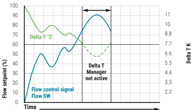
Fig. 32: If the delta T manager was not active, the flow setpoint drives the demand so high that the delta T falls below the desired setpoint of 7.7 K.
