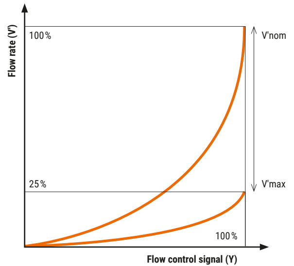
Fig. 26: Flow characteristic in relation to the flow control signal.
