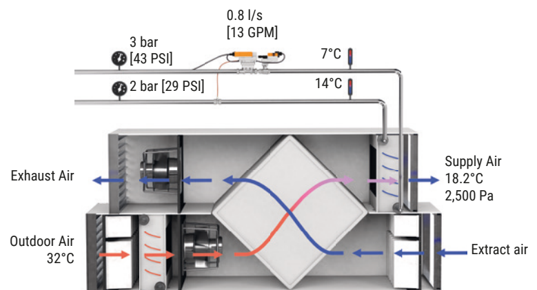
Fig. 64: AHU with delta-T-optimised flow rate.
